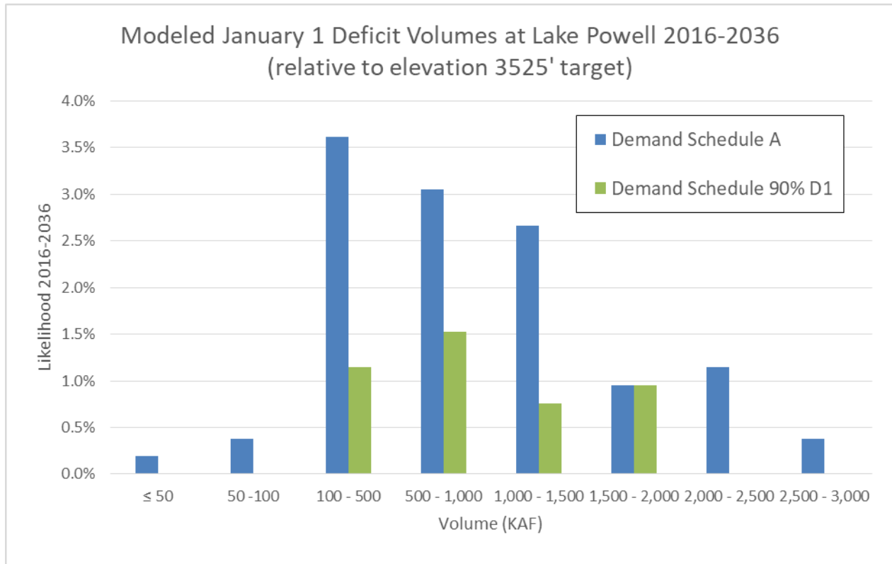
Figure 4. January 1 volumes required AFTER CRSP drought operations to maintain Powell at 3525'. Based on Stress Test (1988-2012) hydrology.
